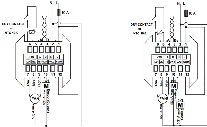
Connection Diagram for 2-Pipe Fan Coil ,
