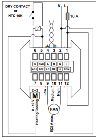
Connection Diagram for 2-Pipe Fan Coil
