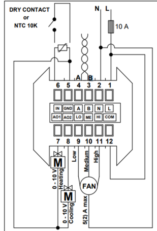
Connection Diagram for 4-Pipe Fan Coil
