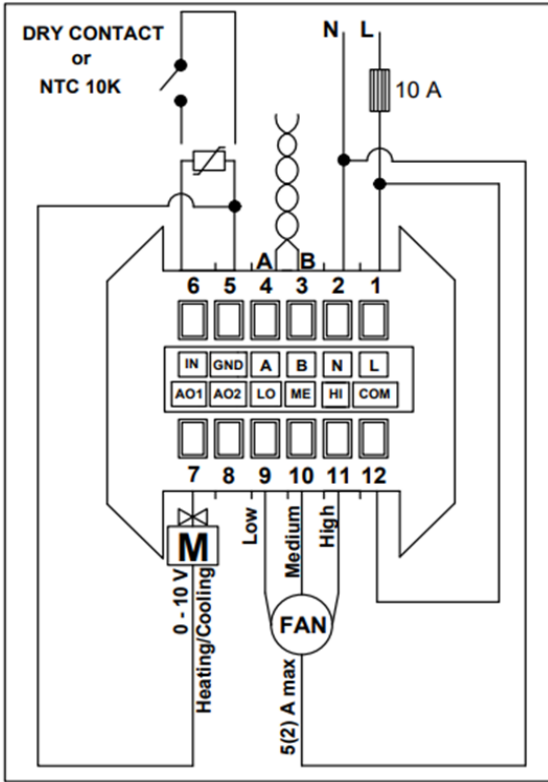
Connection Diagram for 2-Pipe Fan Coil
