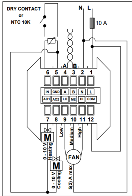
Connection Diagram for 4-Pipe Fan Coil
