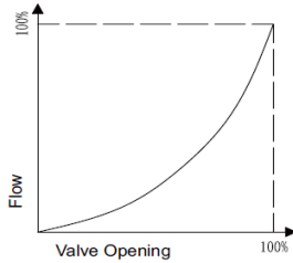
A-AB Equal-percentage Flow Characteristic
