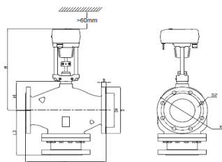
Dimension Figure for PN16 Series
